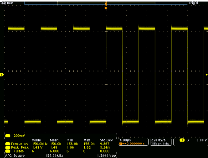
Automated measurement readouts provide repeatable, statistical views of waveform characteristics.
