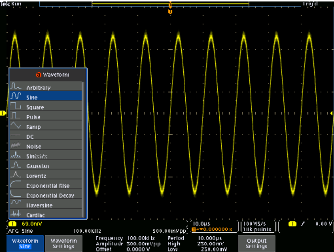
Waveform type selection in the integrated AFG.
