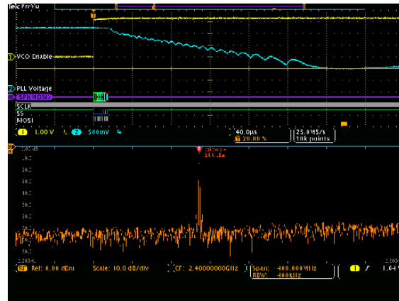
3. Spectrum Time is moved another 160 \mu s to the right. At this point the spectrum shows that the PLL has actually overshoot the correct frequency and gone all the way down to 2.3888 GHz.
